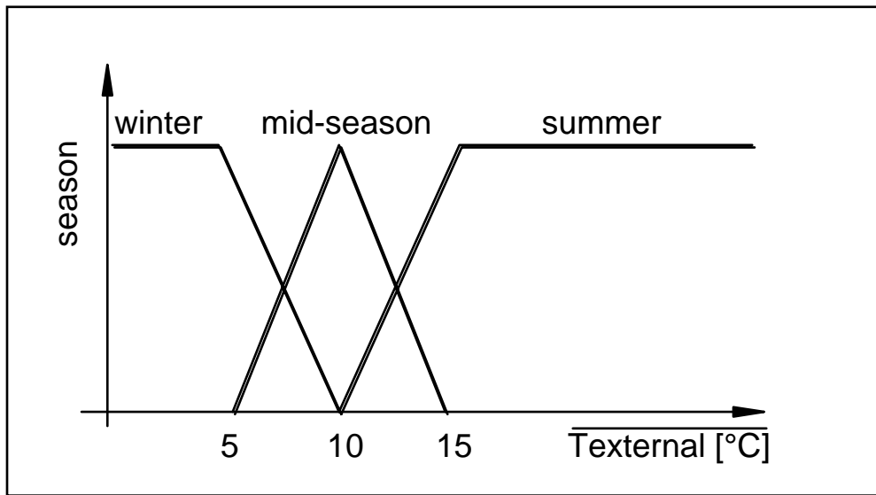
Figure 4: Fuzzy logic variable "season" ( T_{\text{external}} is the average outside temperature during the last 24 hours)
