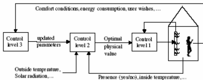
Figure 2.1: Principle block diagram of the three nested control loop levels
